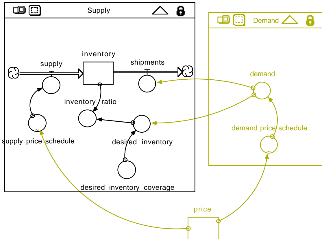
Figure 6: Supply Sector
