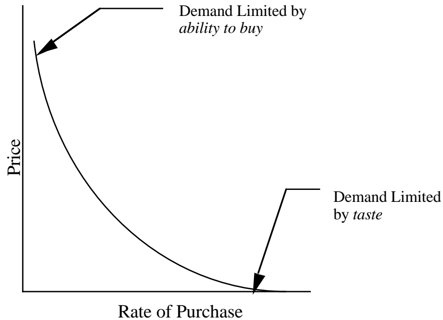
Figure 1: Demand Curve 4
