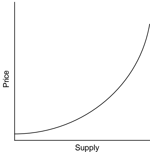
Figure 2: Supply Curve
