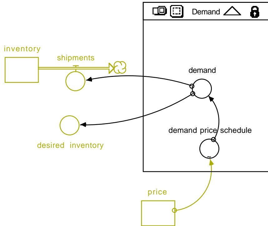
Figure 4: Demand Sector
