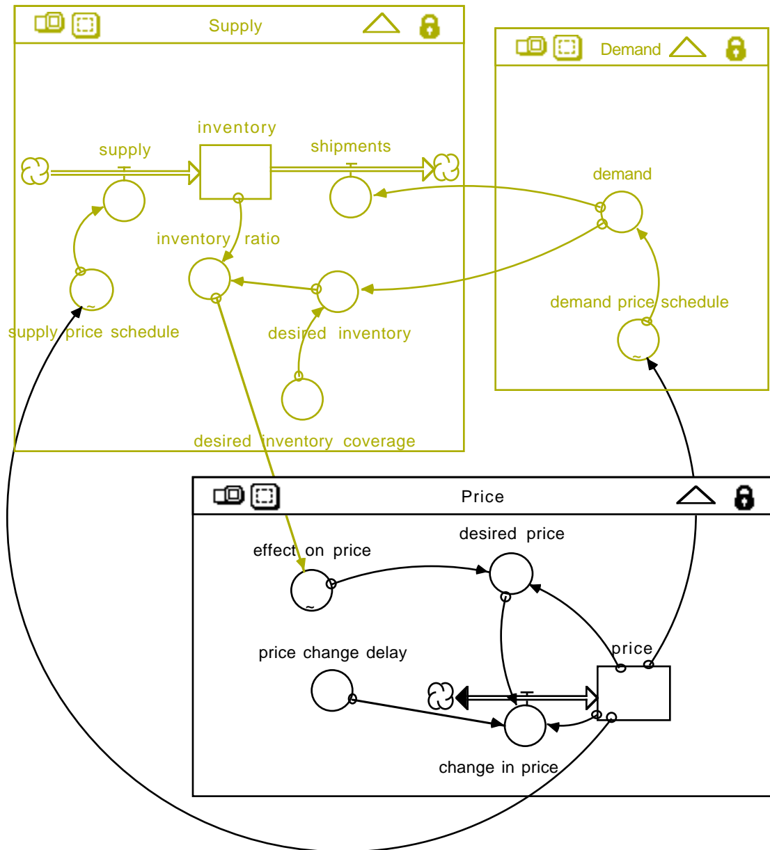
Figure 8: Price Sector
